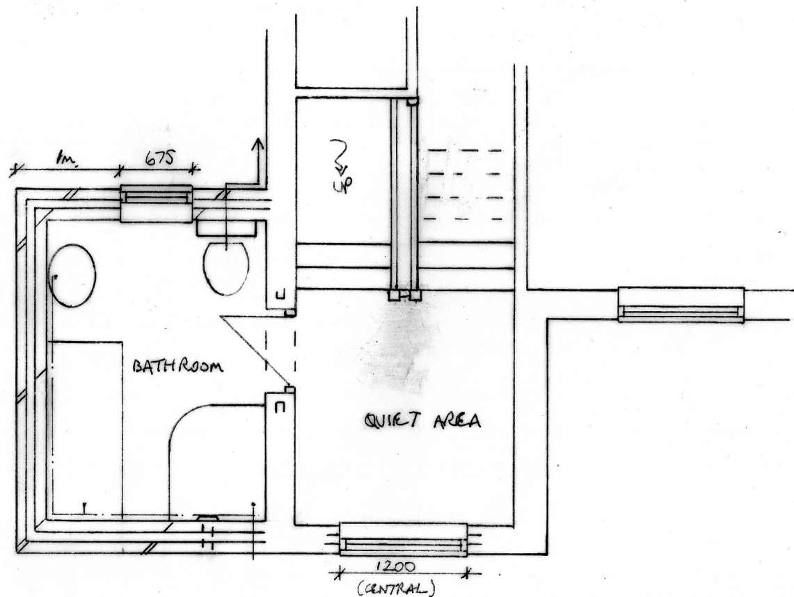
PROPOSED FIRST FLOOR PLAN 1:50
