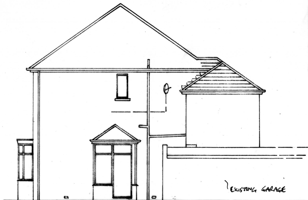
PROPOSED SIDE 1:100
